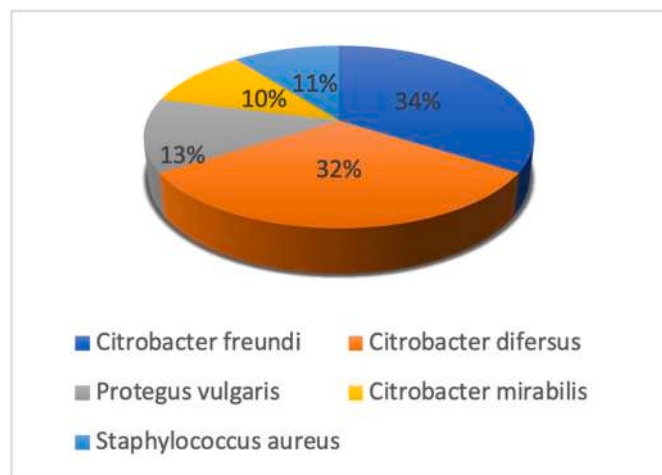
Fig. 2. Bacterial distribution.
